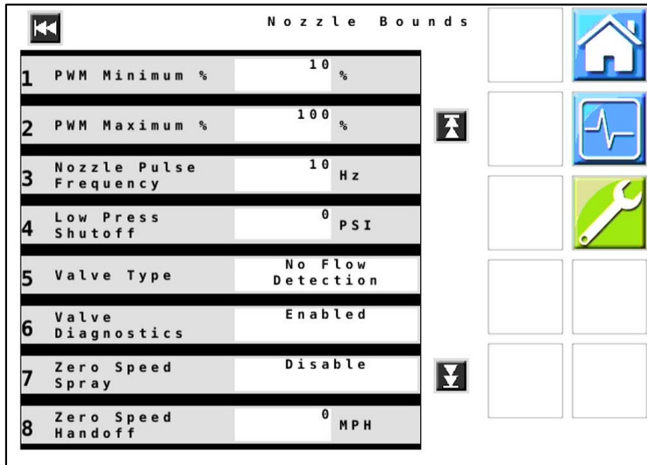
Figure 8 — Nozzle Bounds
