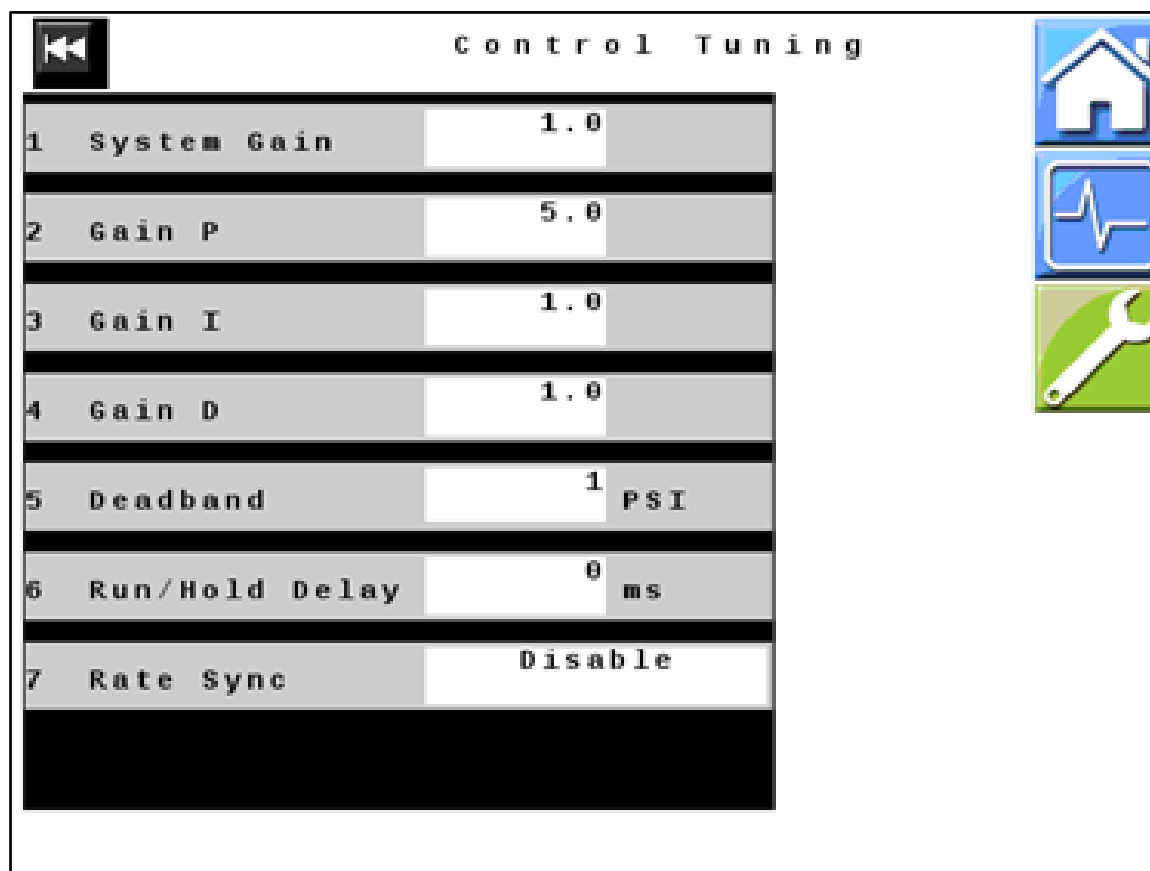
Figure 16 — Control Tuning
