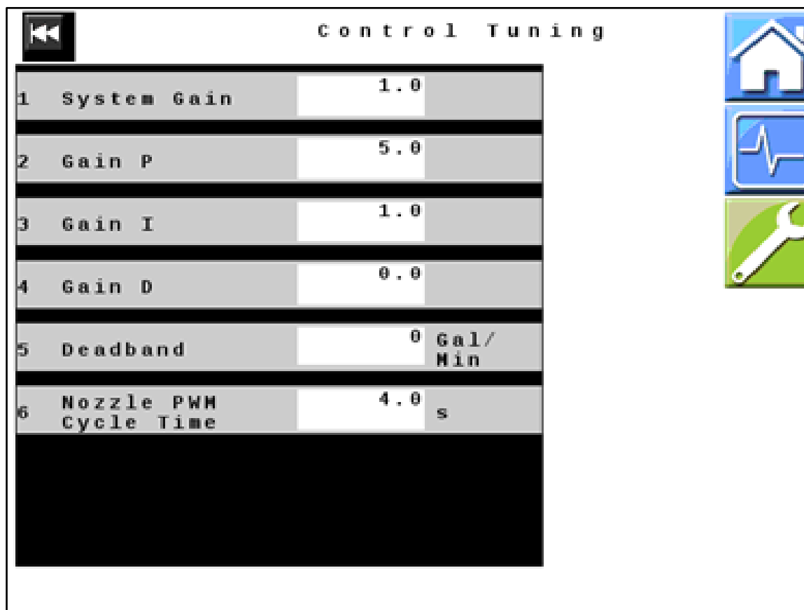
Figure 20 — Control Tuning
