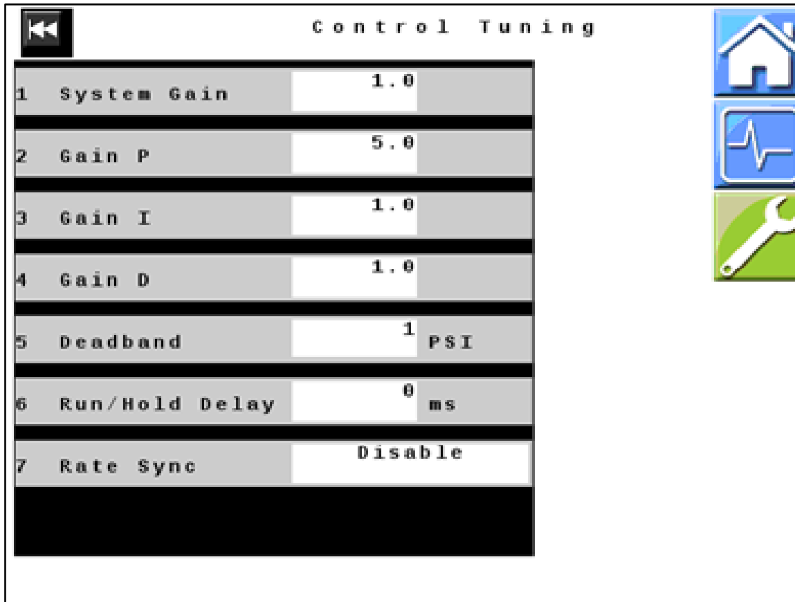
Figure 15 — Control Tuning
