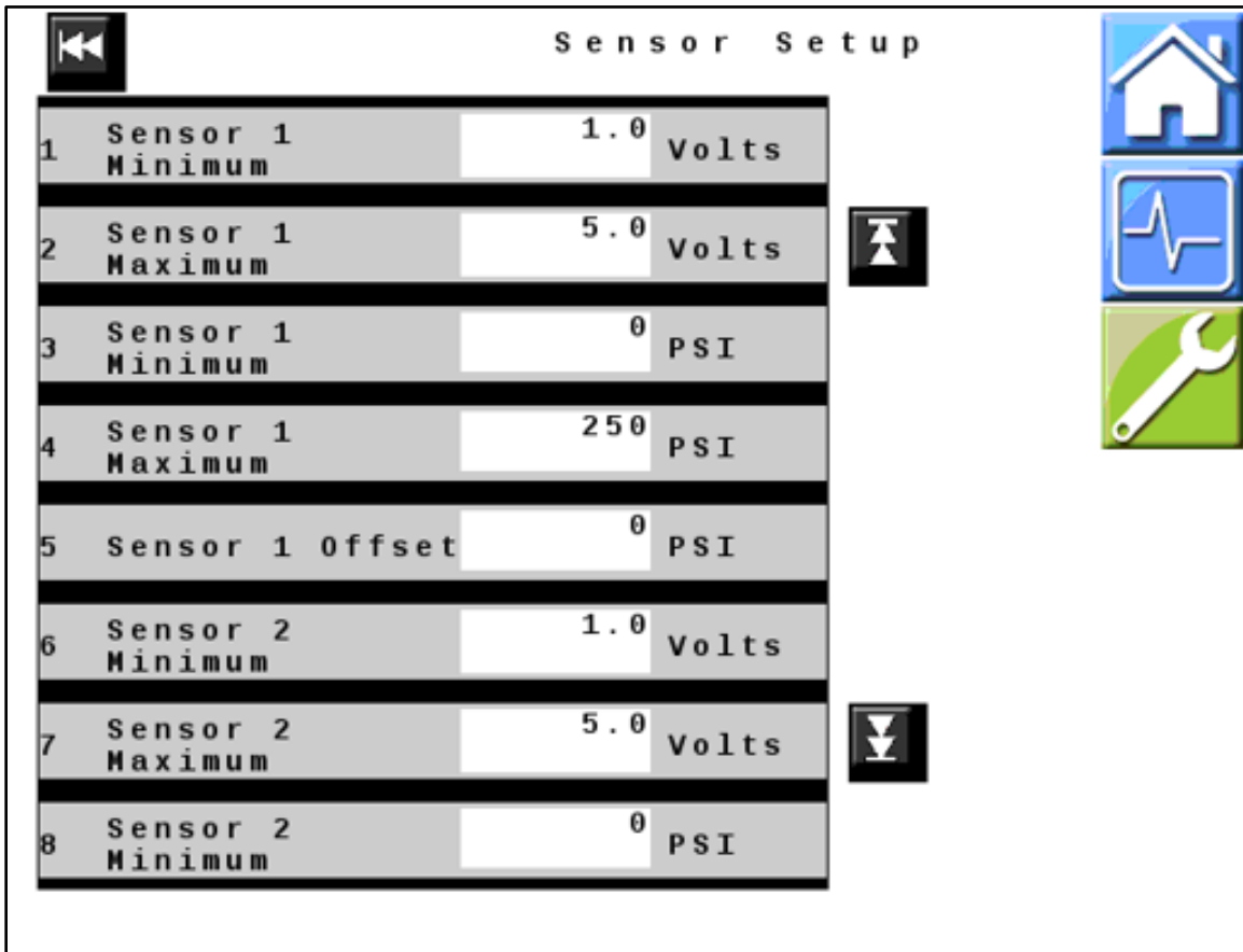
Figure 14 — Sensor Setup Page 1 (OEM Pressure Sensor)
