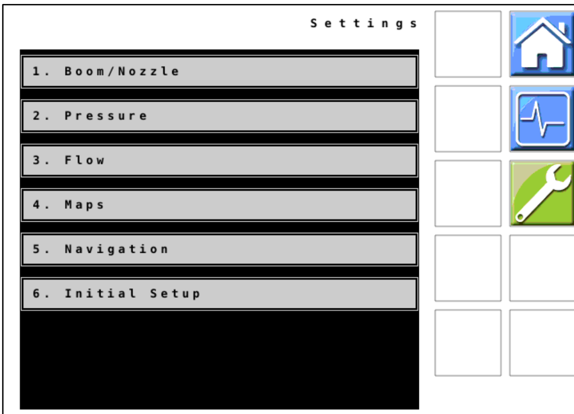
Figure 3 — Settings Menu
